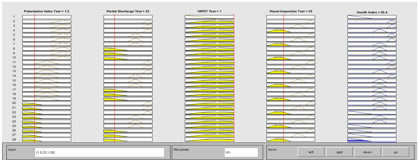
Fig. 13 Fuzzy Inference Diagram for Gen no.1 and Execution of Rule no 28.
