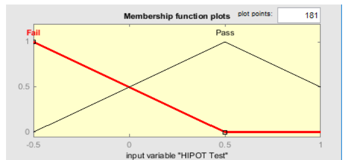
Fig. 8 Membership Functions for High Potential Test.
