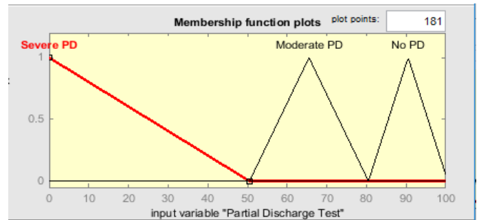
Fig. 7 Membership Functions for PD Test.
