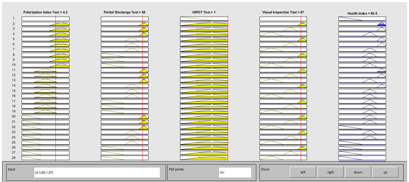
Fig. 12 Fuzzy Inference Diagram for Rule no. 2 and Rule no.11.
