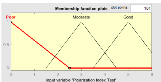
Fig.6 Membership Functions for Polarization Index Test.
