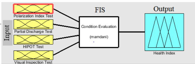
Fig. 3 Fuzzy Inference System (FIS).
