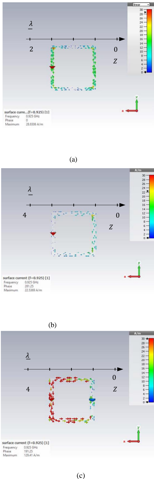
Fig.14 Current distributions(a)typical \lambda/2 dipole,(b) \lambda/4 dipole and (c) \lambda/4 dipole with inductor loading
