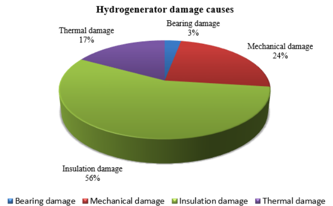
Fig. 1 Cigré Survey on Hydro Generator Failure.
