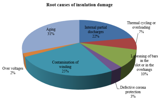
Fig. 2 Root Causes of Insulation Failure.
