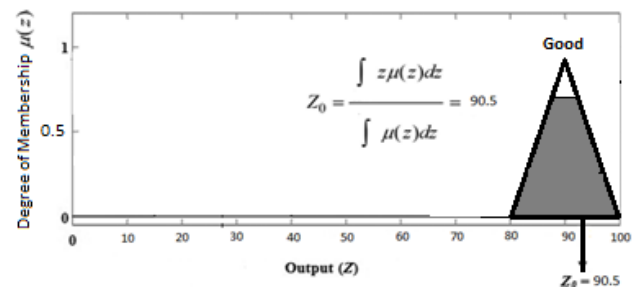
Fig. 11 Determination of HI of Generator by Using Centroid Method.
