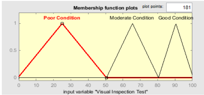
Fig. 9 Membership Functions for Visual Inspection Test.
